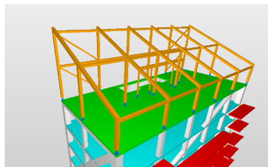
Figure 4 Original pergola design. H=81 m
