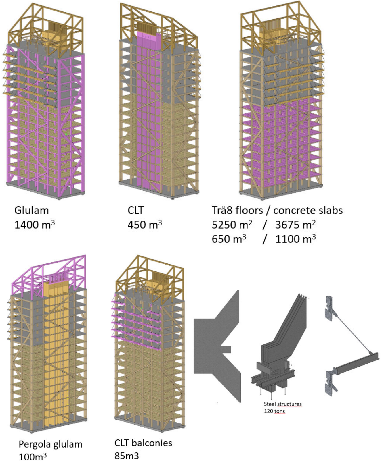
Figure 8 Highlighted volumes used in the building's structure.
