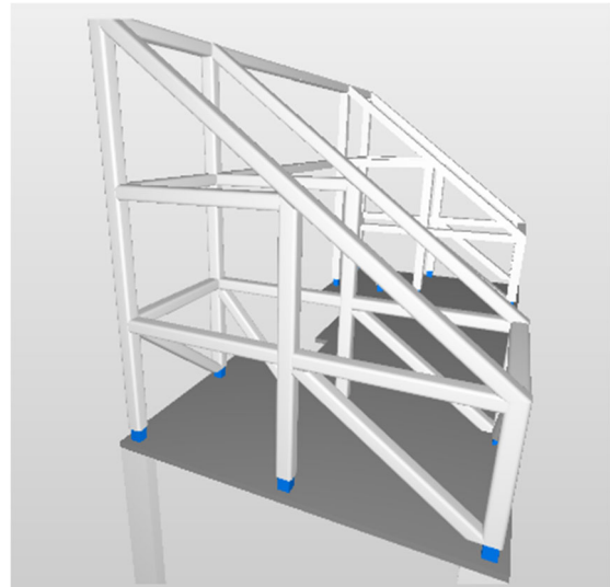
Figure 5 Revised pergola design. H=85,4 m
