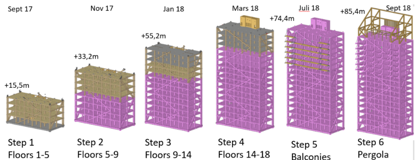
Figure 9 Installation steps
