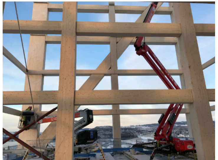
Figure 16 Installation of large glulam structures preassembled on site
